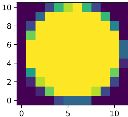
mode='subpixels', subpixels=3
