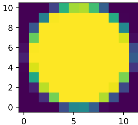
mode='subpixels', subpixels=20
