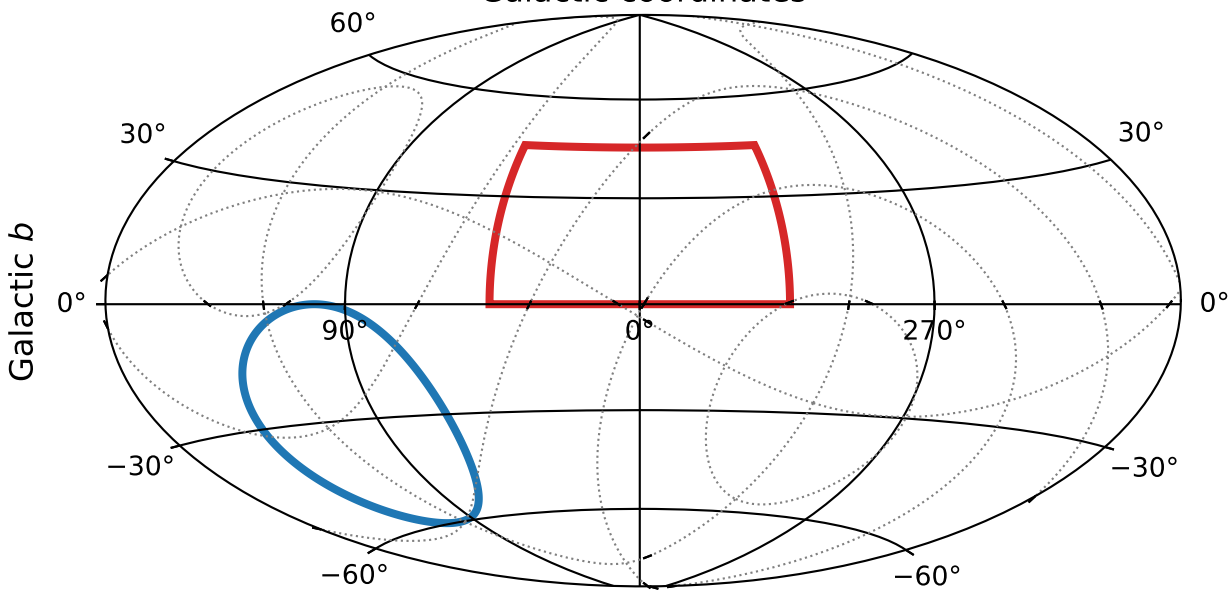
Galactic coordinates
