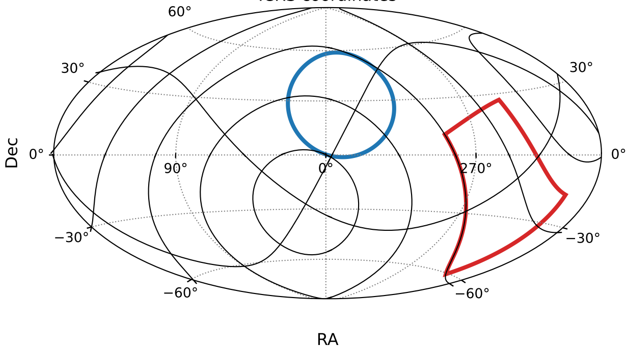
Galactic l ICRS coordinates
