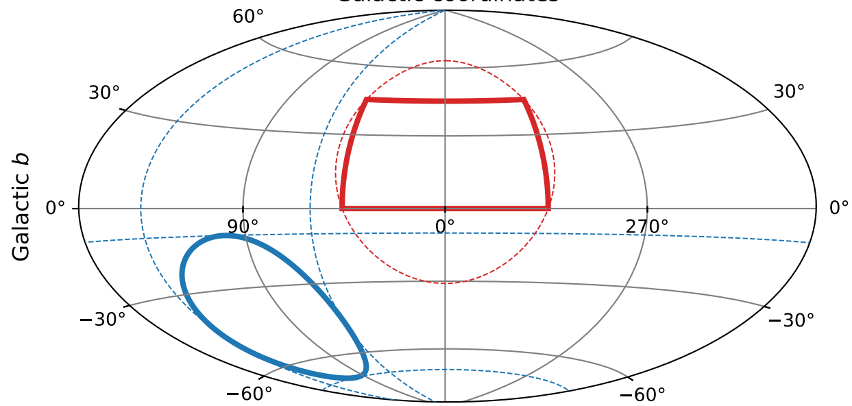
Galactic coordinates
